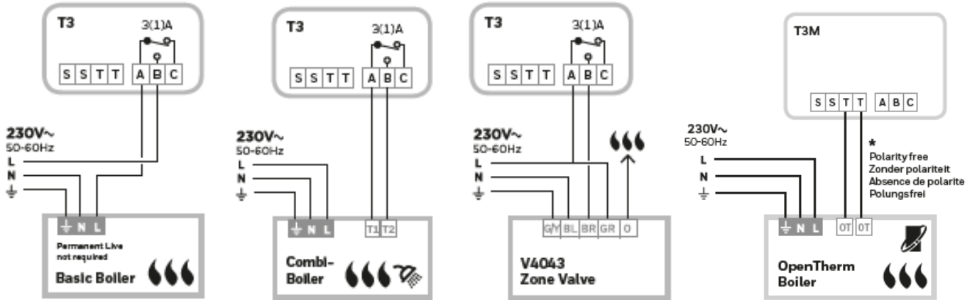
ON/OFF boiler (230V)
