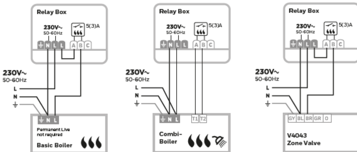
ON/OFF boiler (230V)
